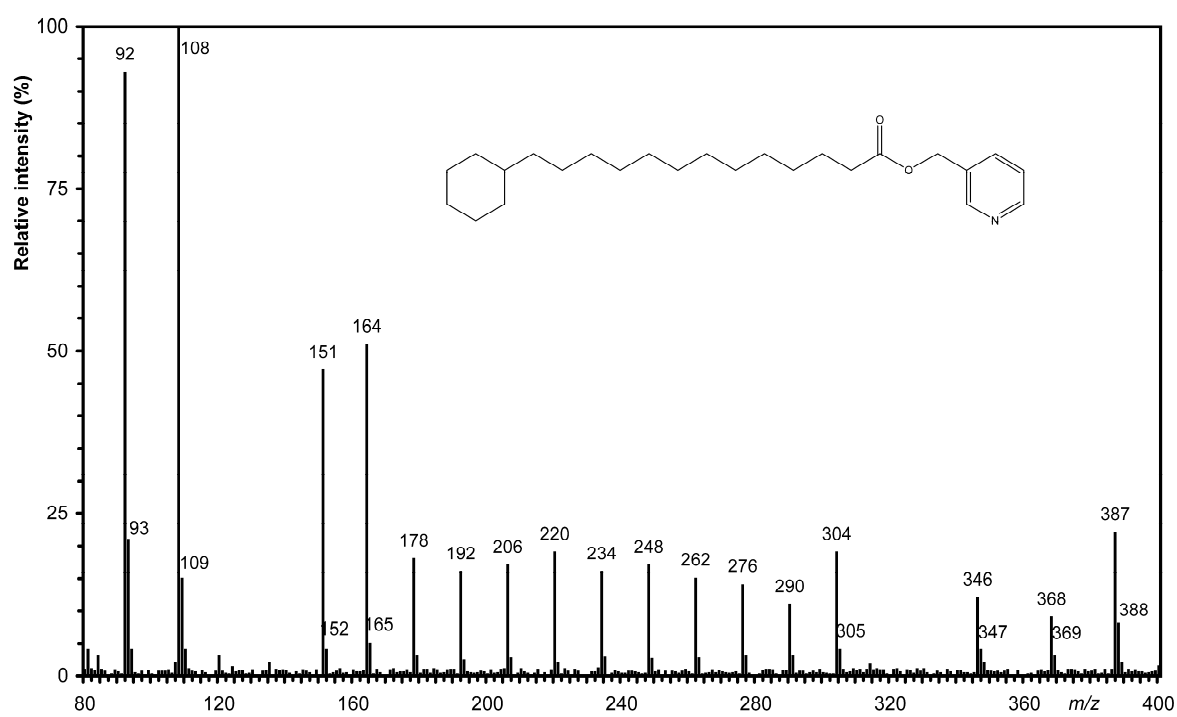
Supplementary Figure S4 Mass spectrum of picolinyl \omega -cyclohexyl tridecanoate
