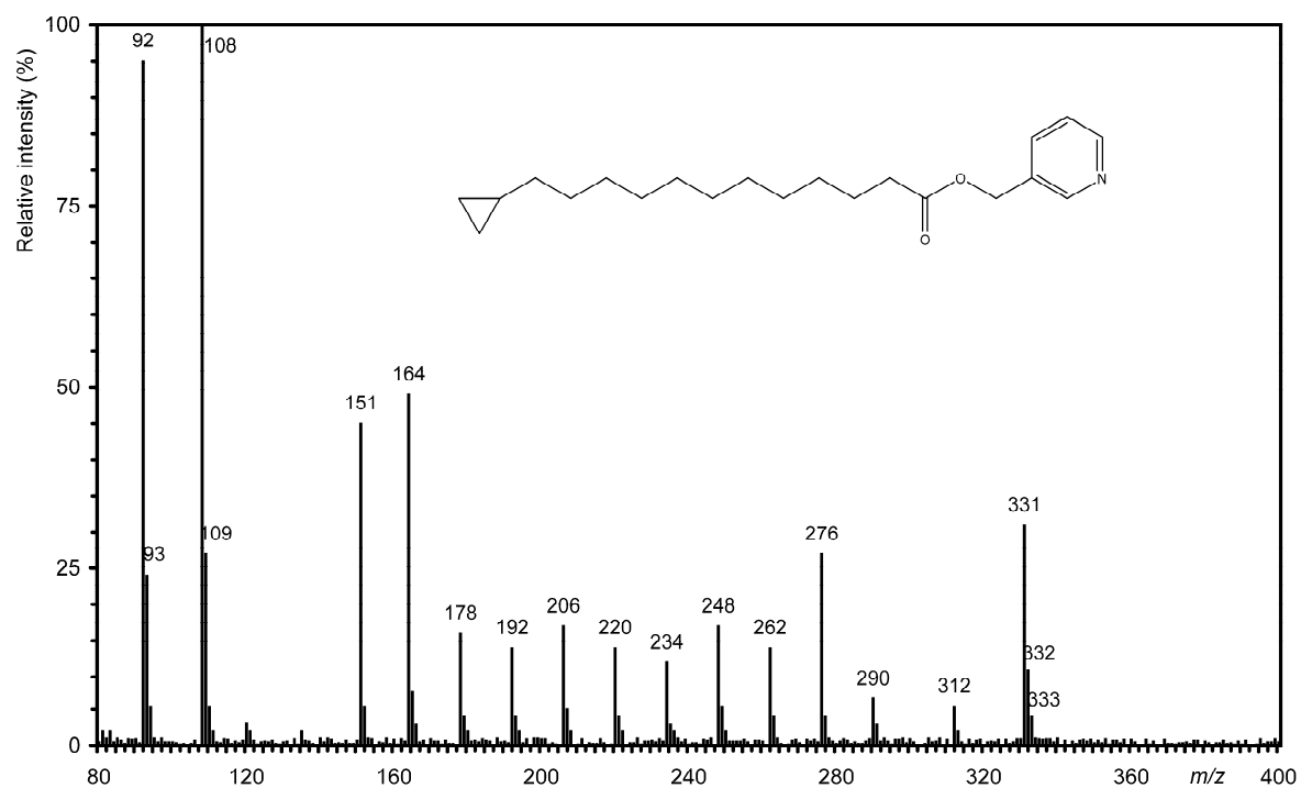
Supplementary Figure S1 Mass spectrum of picolinyl \omega -cyclopropyl dodecanoate
