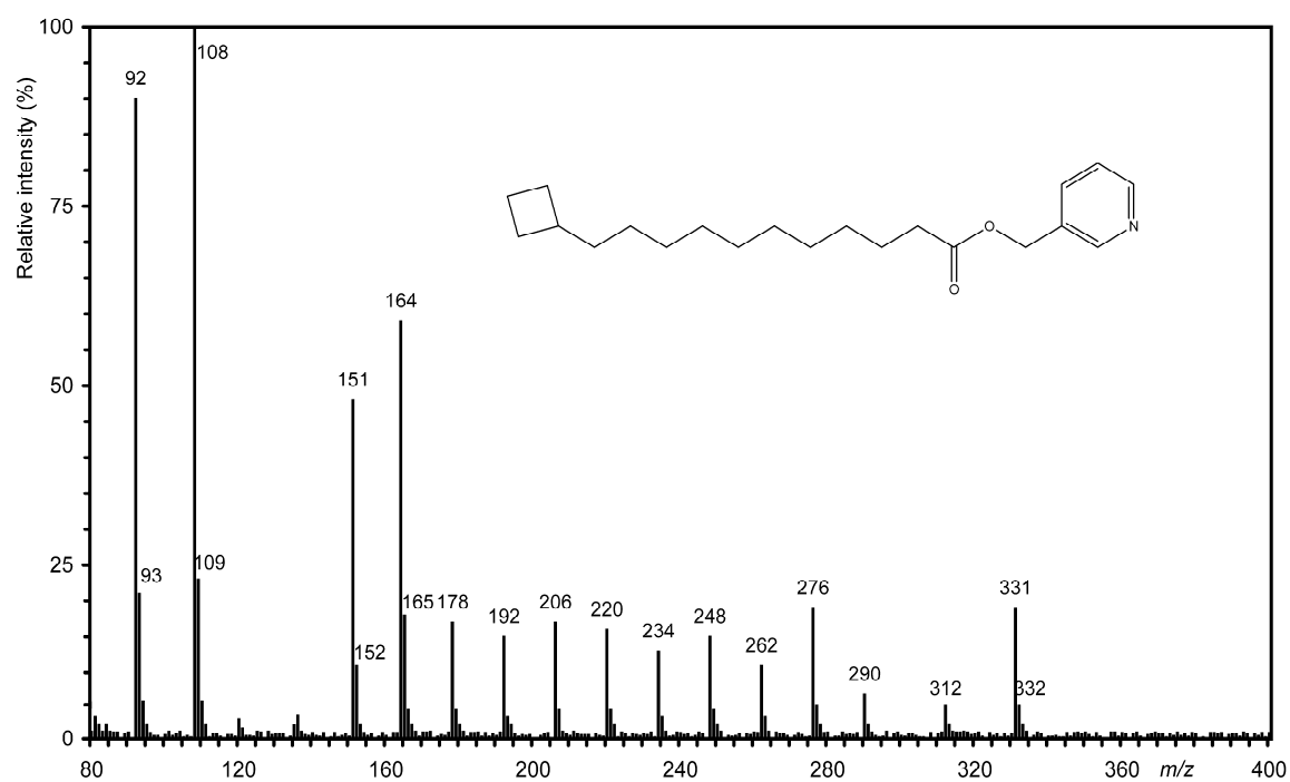
Supplementary Figure S2 Mass spectrum of picolinyl \omega -cyclobutyl undecanoate
