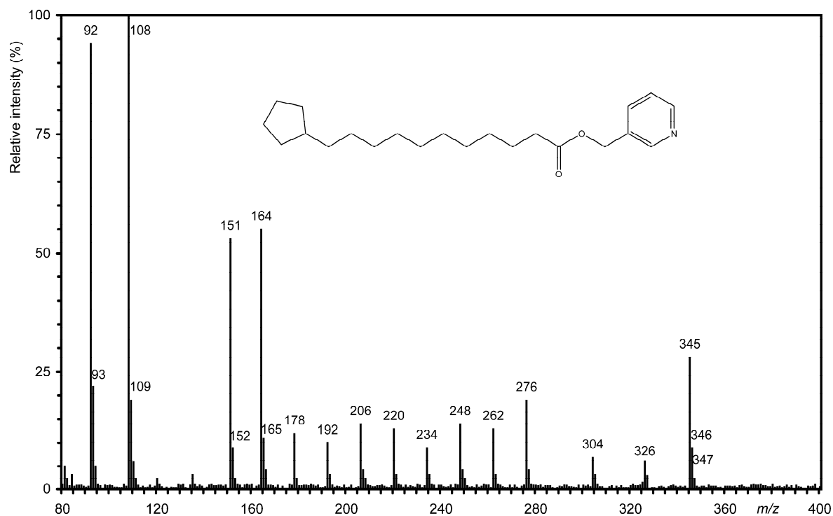
Supplementary Figure S3 Mass spectrum of picolinyl \omega -cyclopentyl undecanoate
