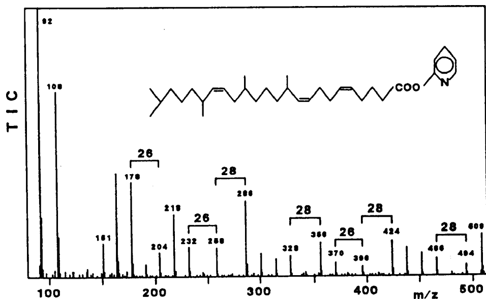
FIGURE 1. Structure and mass spectrum of picolinate of 11,15,19,23-tetramethyl-5,9,17-tetracosatrienoic acid.
