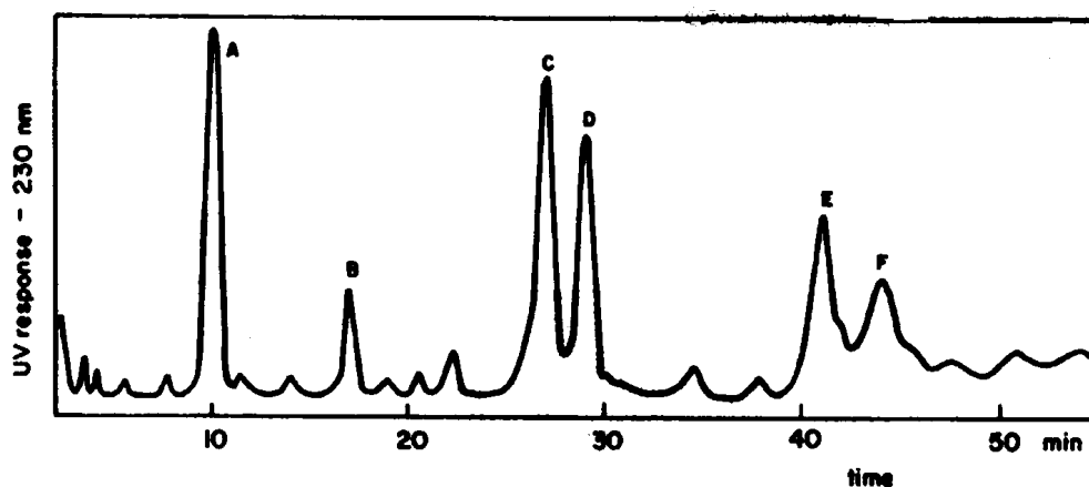
Fig. 1. Preparative HPLC of crude per-O-benzoylglucosylceramides. Peaks A-F are per-O-benzoylglucosylceramides. For structures see Table I and for experimental conditions see text.
