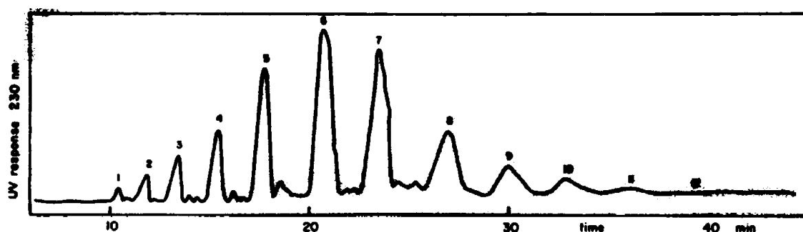
Fig. 3. Semi-preparative RP-HPLC of peak F from Fig. 1. Peaks 1–12 are the molecular species of per-O-benzoylglycosceramides. For structures see Table II and for experimental conditions see text.
