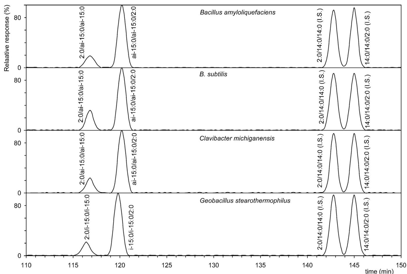
Fig. 6. Chiral separation of natural AcTAG from four bacterial strain including synthesized internal standards (1,2-di-myristoyl-3-acetyl- sn -glycerol and 2,3-di-myristoyl-1-acetyl- sn -glycerol). Two Astec cyclobond TM I 2000 DMP 5 \mu\text{m} \times 25\text{ cm} \times 4.6\text{ mm} were connected in series. The mobile phase was a gradient hexane-2-propanol mixture, with flow rate 0.45 mL/min.
