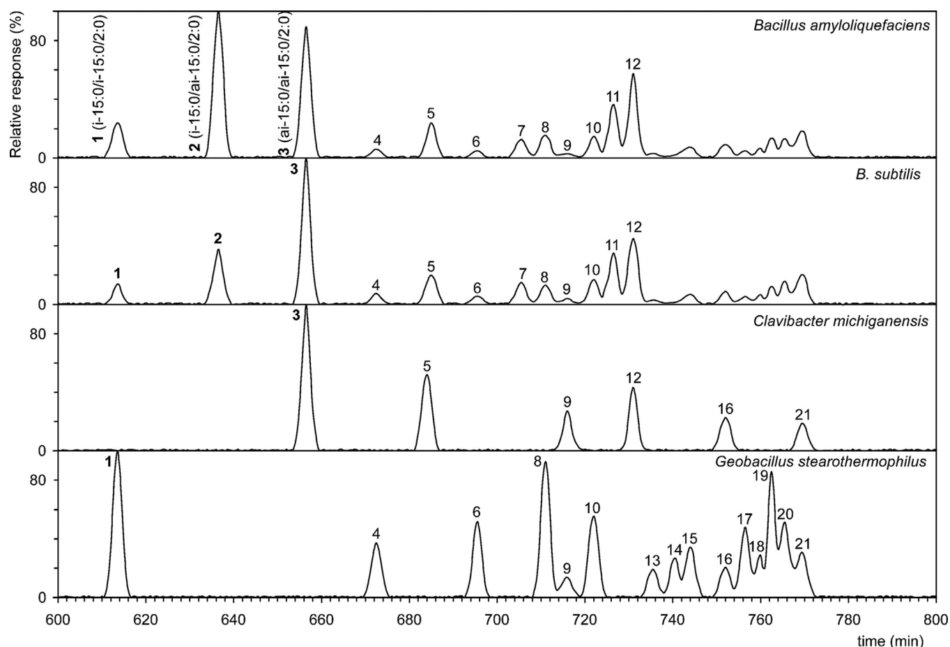
Fig. 5. Separation of AcTAGs obtained after hydrolysis by phospholipase C from four bacteria. The total ion current was filtered and exhibited ions from 200 to 1500 Da. Numbers, see Table 1. Bold numbers - numbers that have been further identified. Three Luna Omega 1.6 \mu m, C18 columns L \times I.D. 150 \times 2.1 mm, connected in series was used with a flow rate of 0.90 mL/min. The gradient program from acetonitrile-2-propanol in ratio 1:1, v/v and acetonitrile-2-propanol in ratio 2:3, v/v was used. The 10% HPLC flow was introduced into the ESI source, and 90% of the flow containing molecular species of AcTAGs was collected manually.
