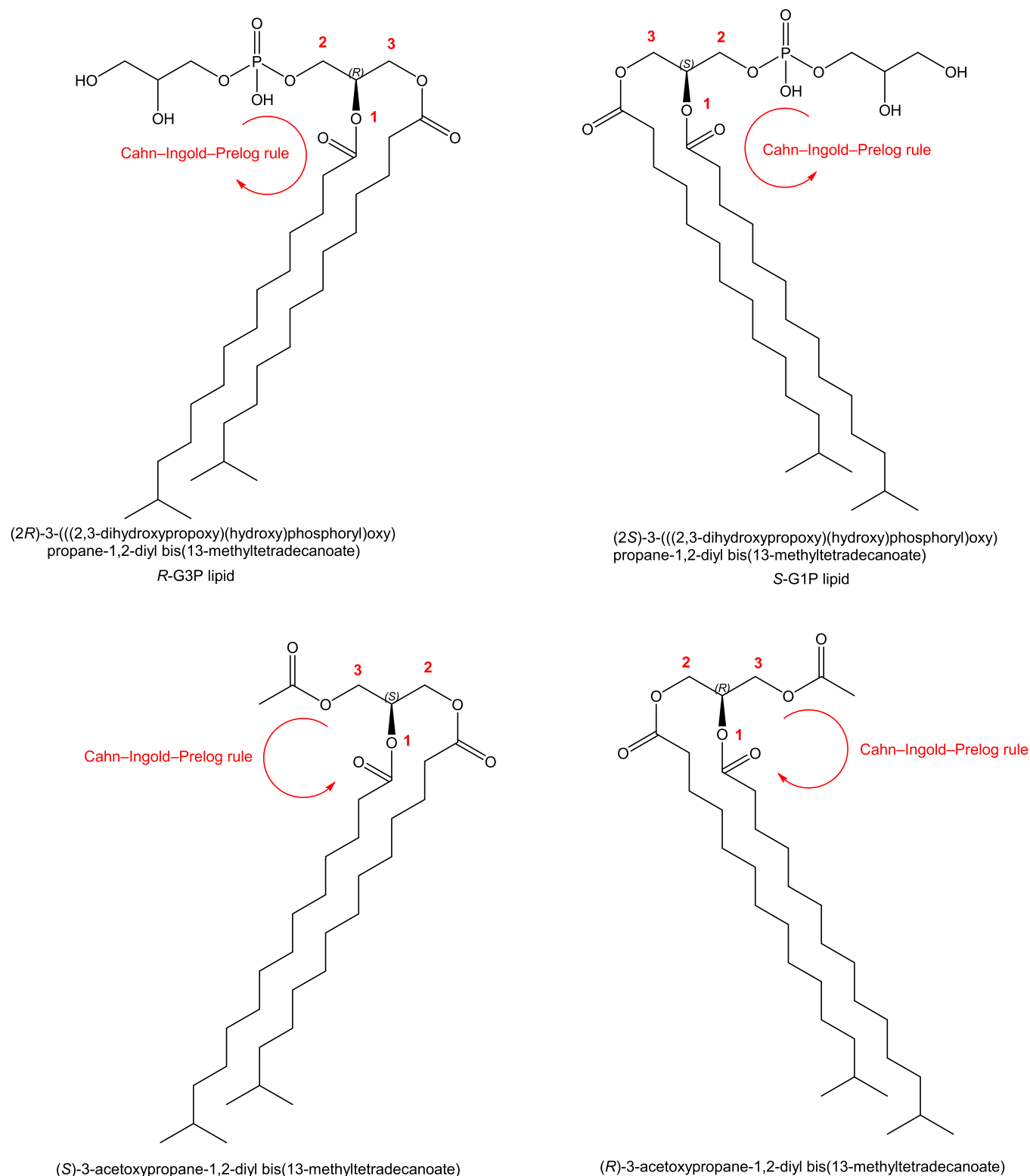
Fig. 8. Use of the Cahn-Ingold-Prelog rule to determine the stereochemistry of PG and AcTAGs, respectively.
