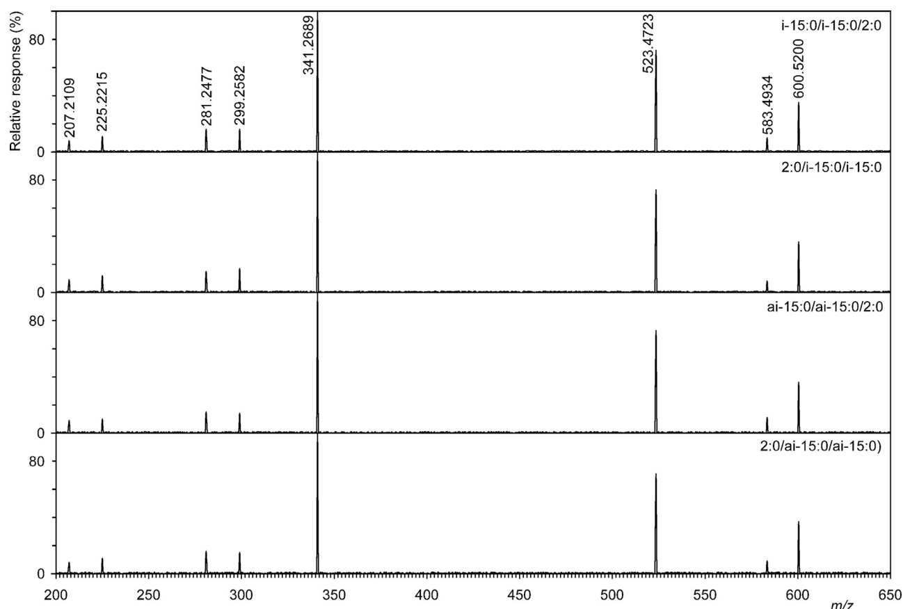
Fig. 7. Tandem mass spectra of four isomers, two pairs of enantiomers (i-15:0/i-15:0/2:0, 2:0/i-15:0/i-15:0, ai-15:0/ai-15:0/2:0, and 2:0/ai-15:0/ai-15:0). For experimental details, see Experimental conditions and explanation of chromatographic behavior, in all figures, including mass spectra, see Results and Discussion.
