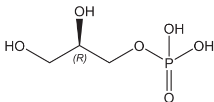
( R )-2,3-dihydroxypropyl dihydrogen phosphate Chemical Formula: C 3 H 5 O 6 P Exact Mass: 172.0137 sn -Glycerol 3-phosphate D-Glycerol 1-phosphate L-Glycerol 3-phosphate
