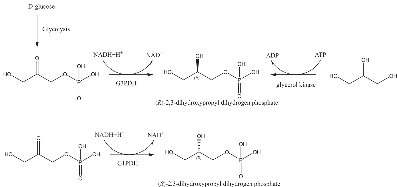
Fig. 2. Biosynthesis of both enantiomers of glycerol-3-phosphate (in bacteria including Eukaryotes) and glycerol-1-phosphate (in Archaea).
