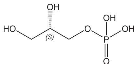
( S )-2,3-dihydroxypropyl dihydrogen phosphate Chemical Formula: C 3 H 5 O 6 P Exact Mass: 172.0137 sn -Glycerol 1-phosphate D-Glycerol 3-phosphate L-Glycerol 1-phosphate
