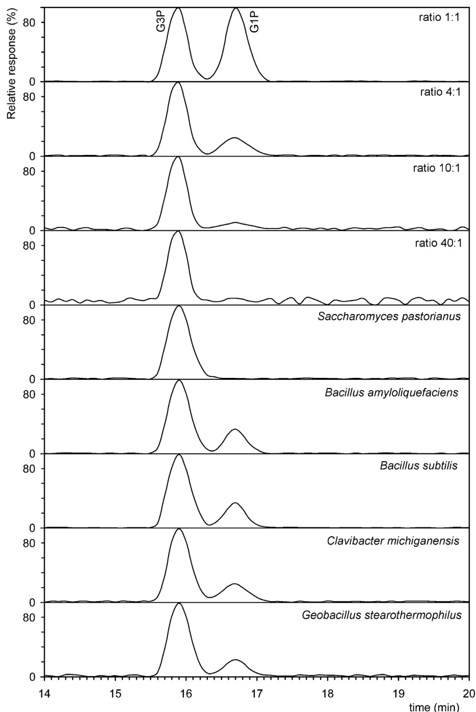
Fig. 3. Four chromatograms of synthetic mixtures of G3P and G1P at different ratios and concentrations are shown. Further, five chromatograms of yeast and bacteria are presented. G3P and G1P were separated by an Astec cyclobond TM I 2000 DMP chiral LC column (5 \mu m, 25 cm \times 4.6 mm). The gradient mobile phase was 5 mM ammonium formate (pH 4.0) and acetonitrile. Glycerol phosphates were quantified by selected ion monitoring (SIM) of ion [M-H]^- at m/z 171.006. The elution order of enantiomers from the chiral column was determined based on the tR of both commercially obtained standards and SIM.
