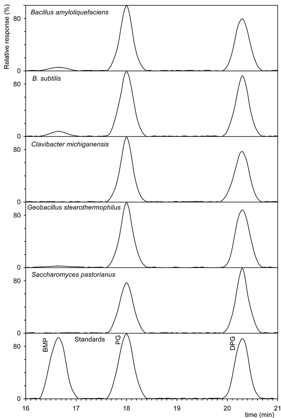
Fig. 4. Hydrophilic interaction liquid chromatography - HILIC/ESI-MS separation of the major lipid classes of five microorganisms, i.e., four bacterial strains and yeast. Standards: bis(monoacylglycerol)phosphate (BMP), phosphatidylglycerol (PG), and diphosphatidylglycerol (DPG). HILIC 250 × 10 mm × 5 μm column was used for semi-preparative HPLC, flow rate of 4.5 ml/min, gradient of the mobile phase containing methanol/acetonitrile/aqueous 1 mM ammonium acetate was used. The eluent from the HPLC column was split so that 2% of the flow was introduced to ESI-MS, and 98% of the flow containing fractions of lipid classes were collected manually.
