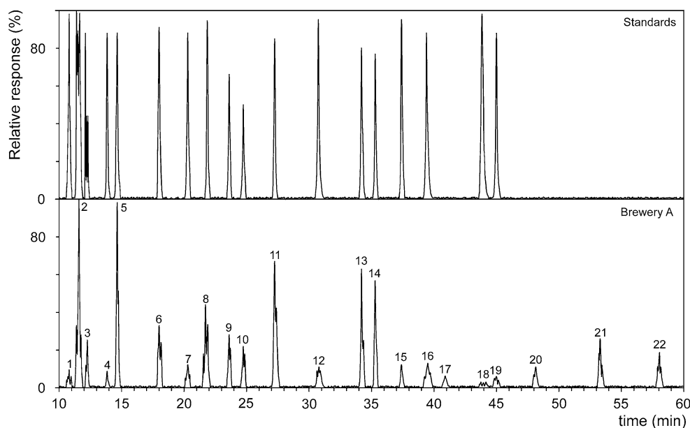
Fig. 2 Separation of both standards and real sample from brewery A by HPLC column with negative electrospray ionization, 1—steryl ester, 2—triacylglycerol, 3—diacylglycerol, 4—unesterified fatty acid, 5—sterol, 6—phosphatidylglycerol, 7—cardiolipin; 8—phosphatidylcholine, 9—dimethyl-phosphatidylethanolamine,
