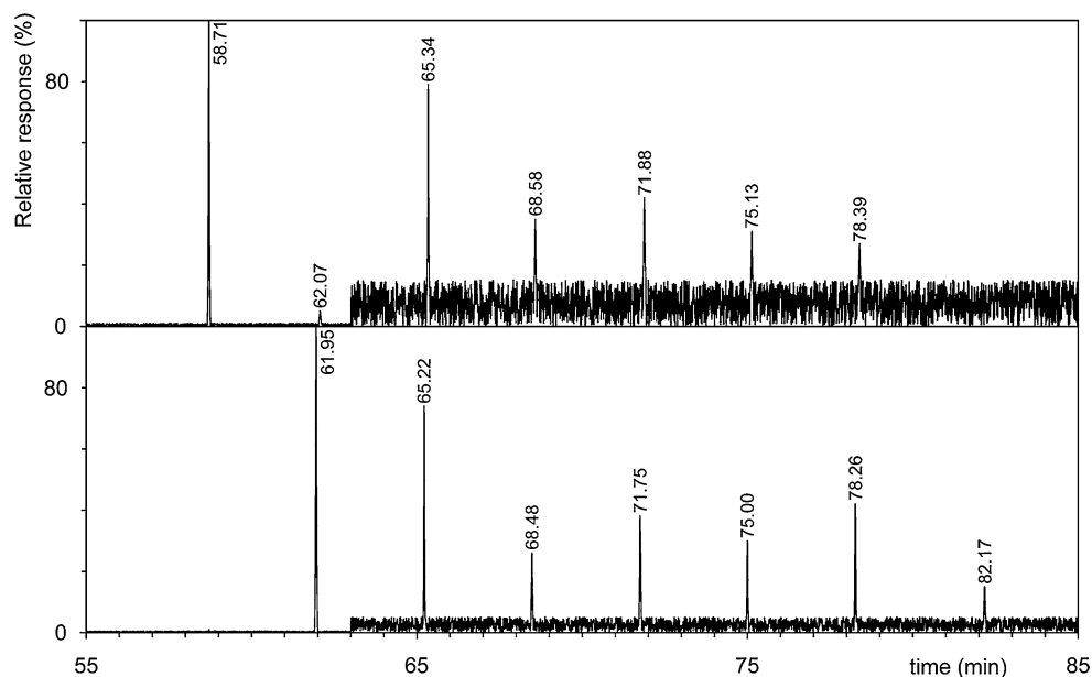
Fig. 1 GC–MS analysis of total FAME as DMDS adducts obtained from yeast from brewery A shows a selected-ion monitoring chromatogram for ions at m/z 145 (top trace) for \omega -7 FA, and at m/z 173 (lower recording) for \omega -9 FA
