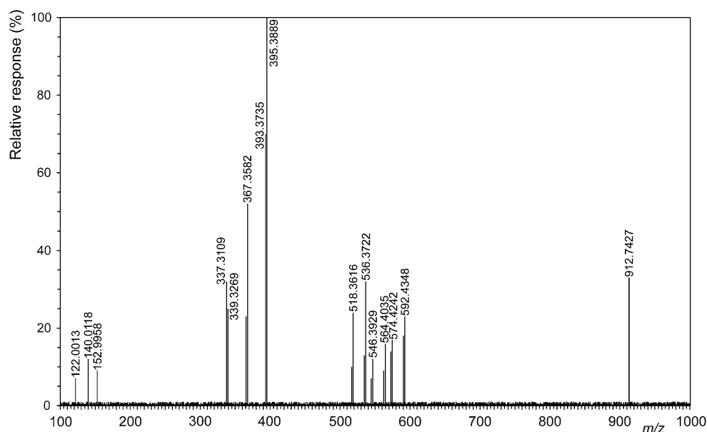
Fig. 3 High resolution tandem mass spectra of [M-H]^- ions at m/z 912.7427 (molecular species of phosphatidylethanolamine 26:0/22:1, 24:0/24:1 and 26:1/22:0) from lipid extract of yeast from brewery Δ
