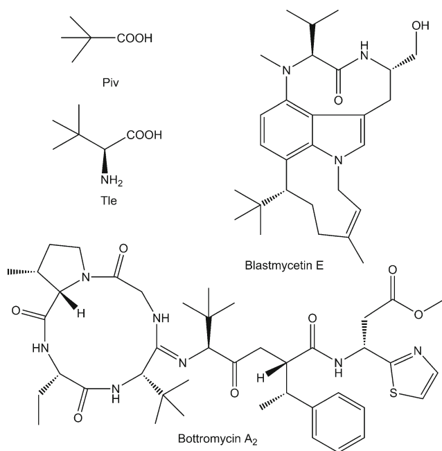
Fig. 1 Natural compounds with t -butyl group
