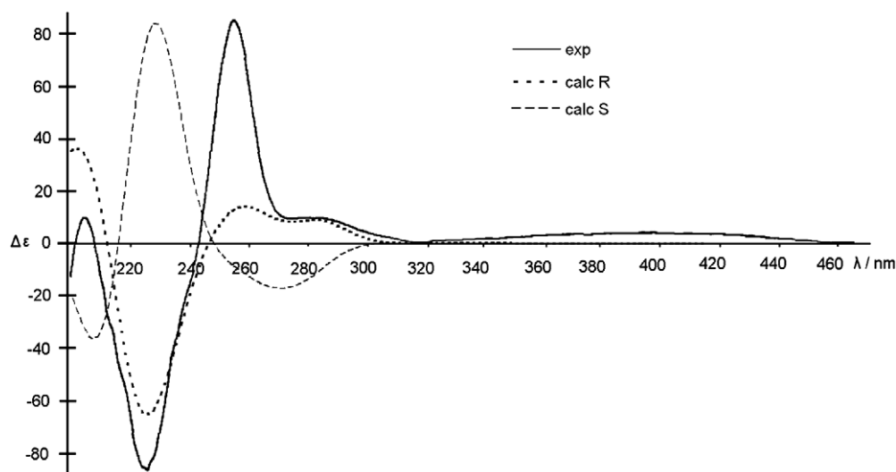
Fig. 2. B3LYP/6-31G*-calculated CD spectrum for ( R )- 1 , ( S )- 1 , and experimental CD spectrum of 1 .
