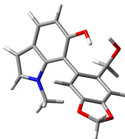
Fig. 3. Model of ( R )-6-hydroxy-galanthindole ( 1 ) shows that rotation about the 7,5' bond is hindered.
