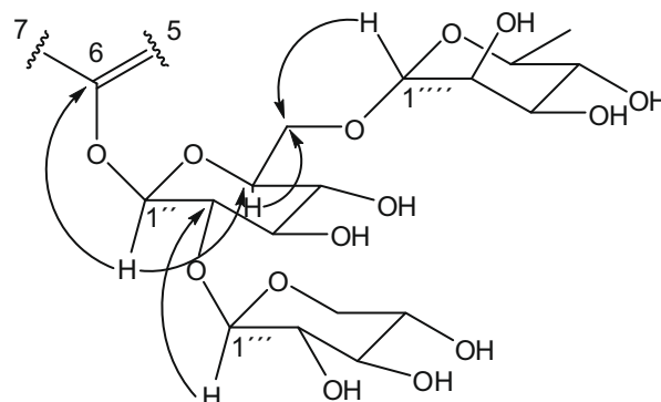
Fig. 4. The key HMBC correlations of saccharide moiety of glycoside 4 .
