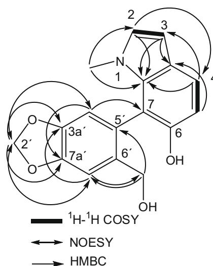
Fig. 1. Structure of the new compound ( 1 ); only important HMBC, COSY, and NOESY correlations are shown.
