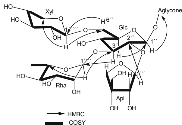
Fig. 4. The HMBC and COSY correlations of tetrasaccharide moiety of glycoside 4 , only important correlations are showed.
