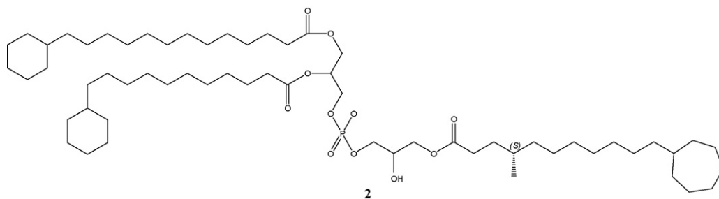
Fig. 4. Structure of acylphosphatidylglycerol [1-(13-cyclohexyltridecanoyl)-2-((S)-11-cyclohexylundecanoyl)-sn-glycero-3-phospho-(3'-(11''-cycloheptyl-4''-methylundecanoyl))-1'-sn-glycerol]; brc19:0-c19:0/c17:0-PG] ( 2 ).
