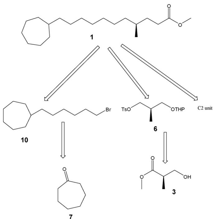
Scheme 1. Structure of the acid [( S )-11-cycloheptyl-4-methylundecanoic (brc19:0)], and its retrosynthetic analysis.
