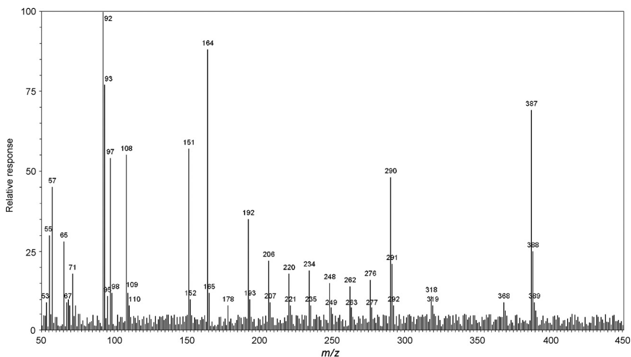
Fig. 1. Electron ionization mass spectrum of (S)-11-cycloheptyl-4-methylundecanoic (brc19:0) picolinyl ester of acyl-PG from Alicyclobacillus acidoterrestris .
