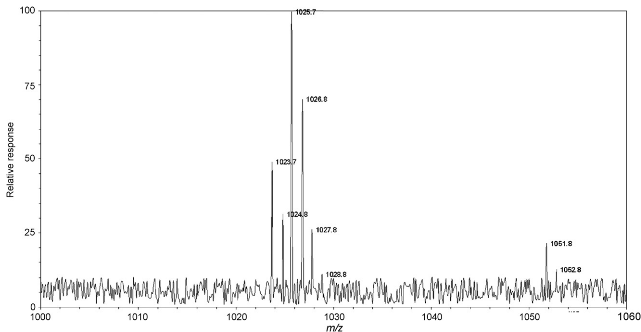
Fig. 2. Negative ion electrospray mass spectrum of deprotonated molecular ions of acyl-PG from A. acidoterrestris .
