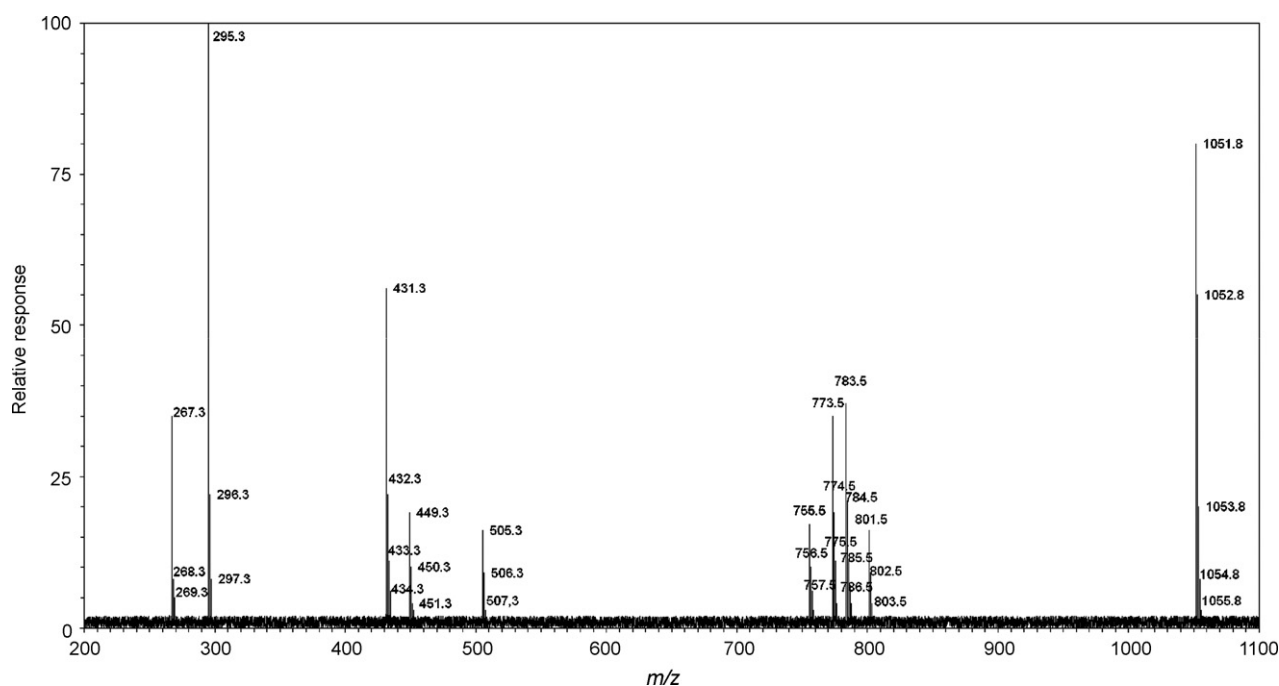
Fig. 3. The tandem quadrupole ESI product-ion spectra of the [M-H]^- ion of brc19:0-c19:0/c17:0-PG at m/z 1051.8.
