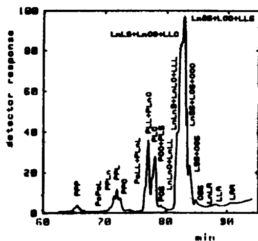
Fig. 1. GLC of triacylglycerols.
