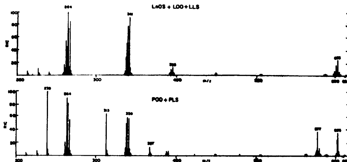
Fig. 2. EI-MS of LnOS + LOO + LLS and POO + PLS.
