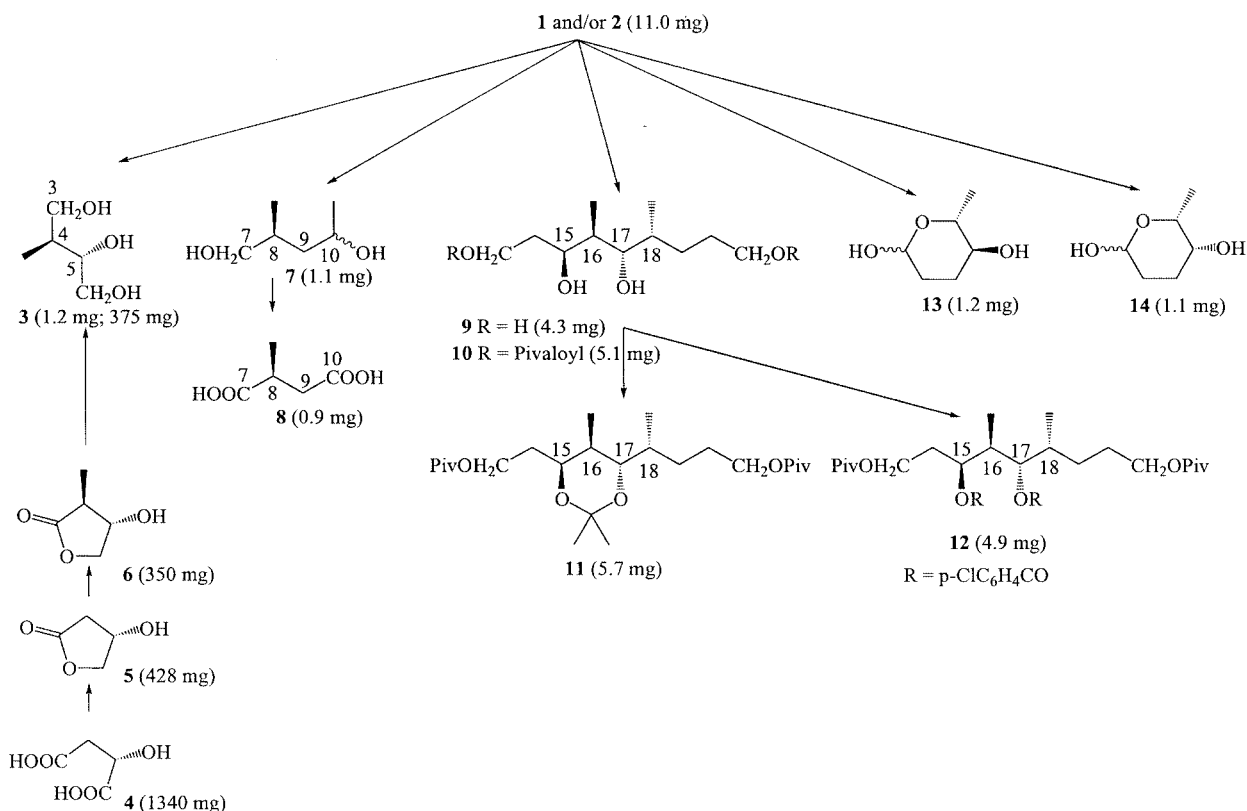
Figure 4. Reaction schema of degradation compounds from glycoside 1 ( 2 ) and synthesis of standard (2 S ,3 S )-3-methyl-butane-1,2,4-triol ( 3 )
