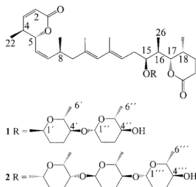
Figure 1. Structure of new glycosides, i.e. lycoperdinoside A and B ( 1 and 2 ) from slime mold Enteridium lycoperdon
