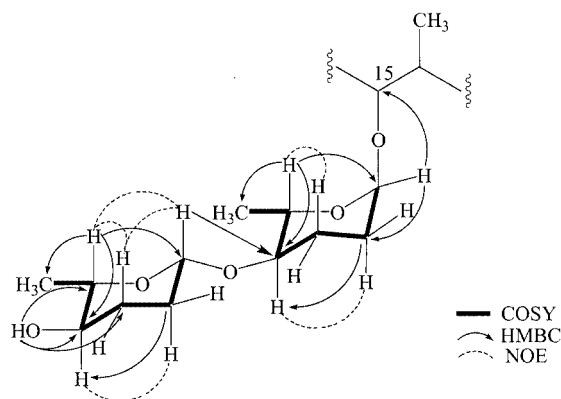
Figure 3. The H-H COSY, HMBC and NOE correlations of saccharidic part of lycoperdinoside A ( 1 )
