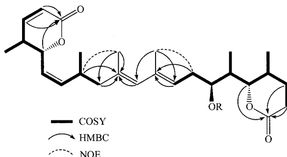
Figure 2. The H-H COSY, HMBC and NOE correlations of aglycone part of lycoperdinoside A ( 1 )
